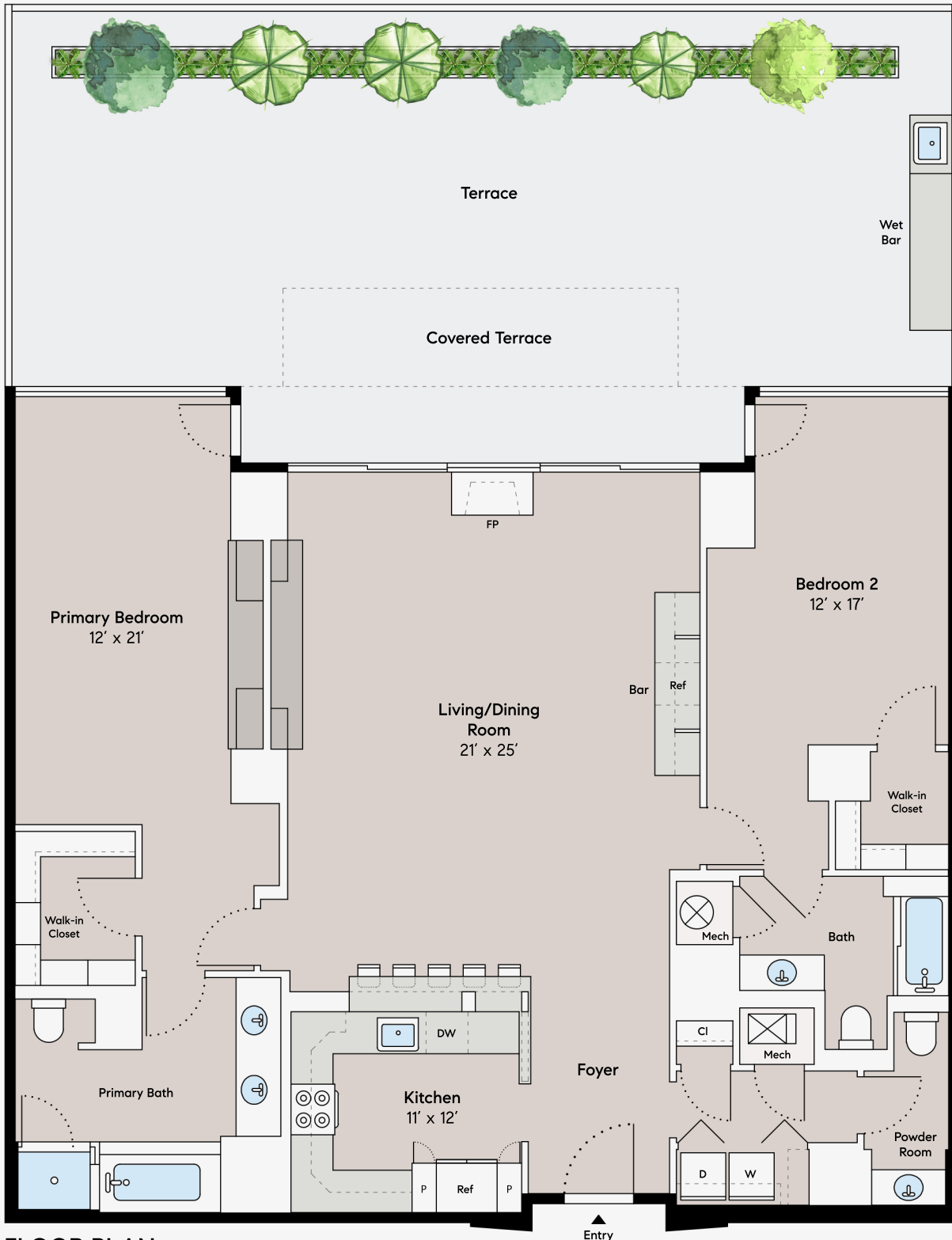
FLOOR PLAN
